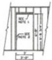
TYPICAL EXTERIOR DOOR FRAMING DETAIL N.T.S.
