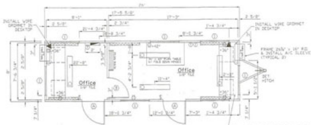
FLOOR PLAN
